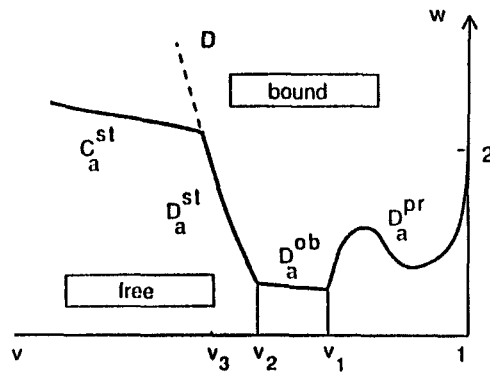
FIGURE 1 Schematic phase diagram for the shape transformations of a vesicle in the presence of an attractive surface. The thick line represents transitions between a free and a bound state, the thin full lines between two different free states, and the thin broken line ( D ) between two different bound states. The parameters w and v are the reduced adhesion energy and the reduced volume as defined in the text.
